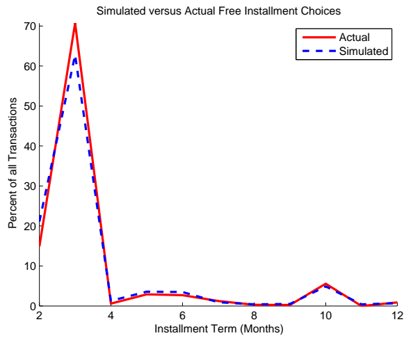
Figure 29: Predicted versus Actual Free Installment Choices
