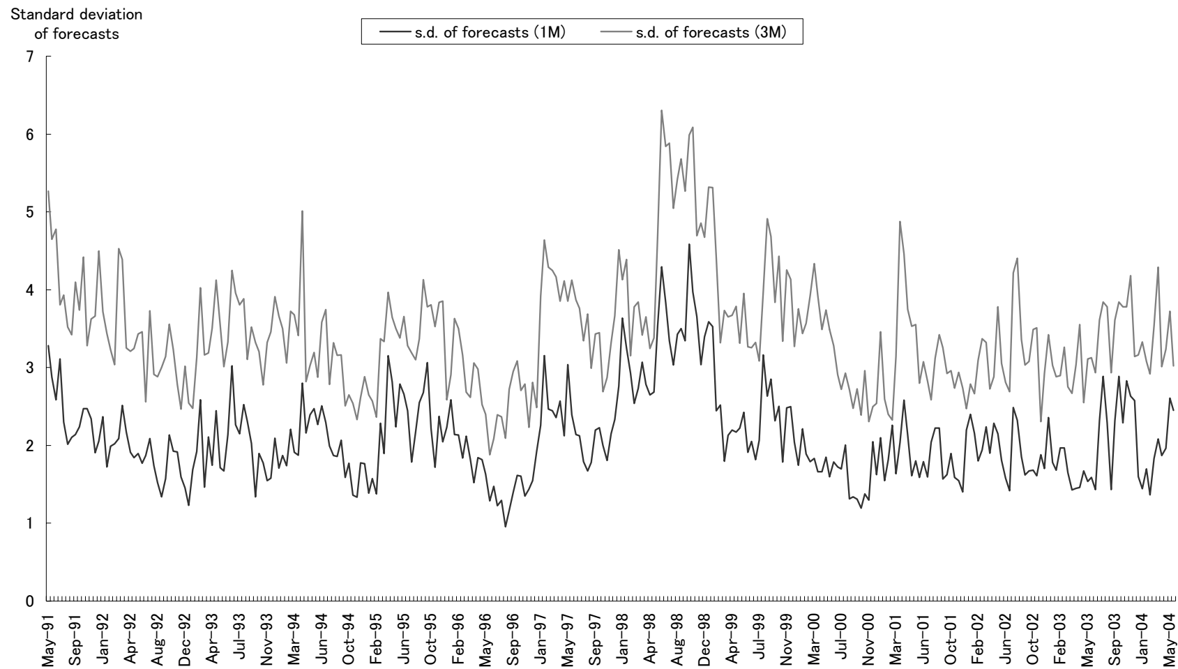
Figure 3. Expectation heterogeneity
