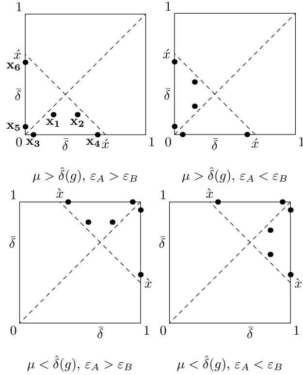
Figure 3: Nash equilibria in perturbed games
