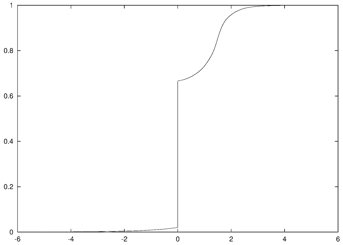
Figure 2: The Limiting Null Distribution of V_T
