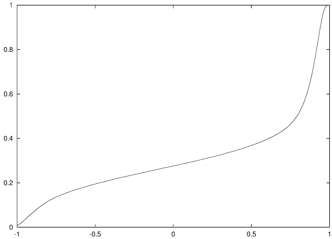
Figure 1: Finite Sample Distribution of the MLE of the AR Parameter for the ARIMA Model
